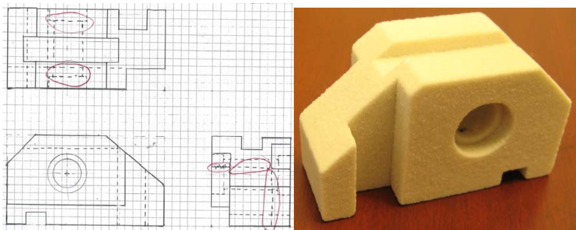
Figure 4. Student's modified multiview drawing (left) based on input from the RP model (right).
