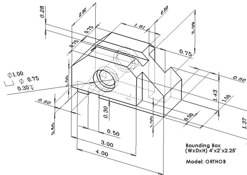
Figure 3. Trimetric view of model used to generate multiview drawing. Note: Location of counterbored holes has been omitted for clarity.
